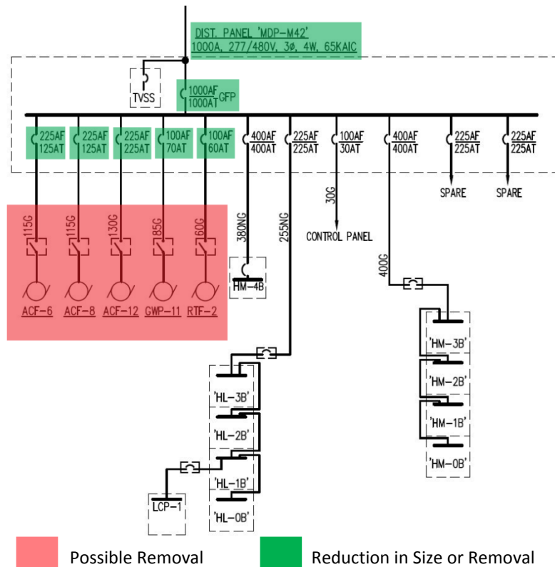
Figure 6: Single line diagram changes
