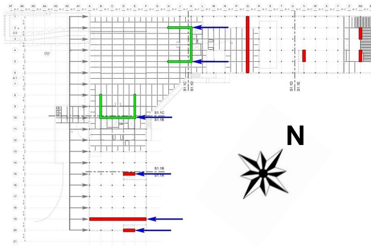
Figure 14: Existing Lateral System Placement
