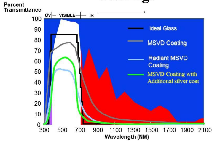
Figure 9: MSVD Coating performance graph courtesy of Darijo Babic, PPG
